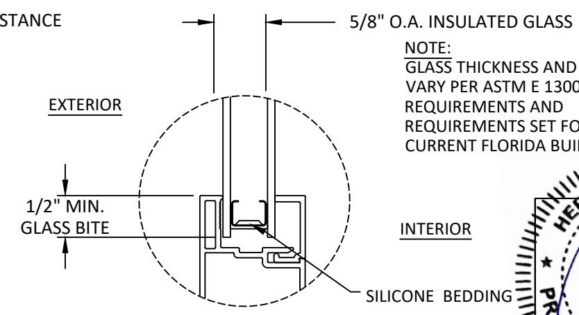
GLAZING DETAIL
