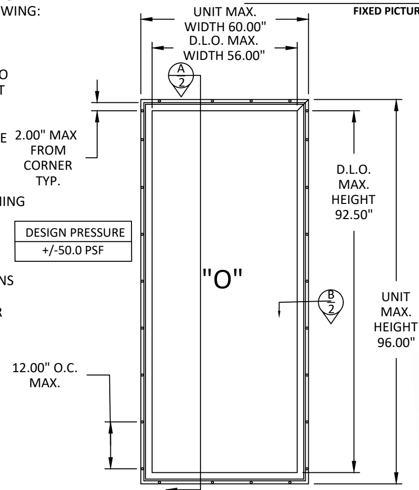
ELEVATION AND ANCHOR LAYOUT FIXED PICTURE WINDOW
