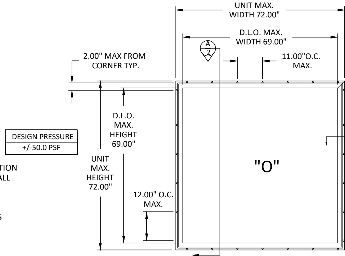
ELEVATION AND ANCHOR LAYOUT
